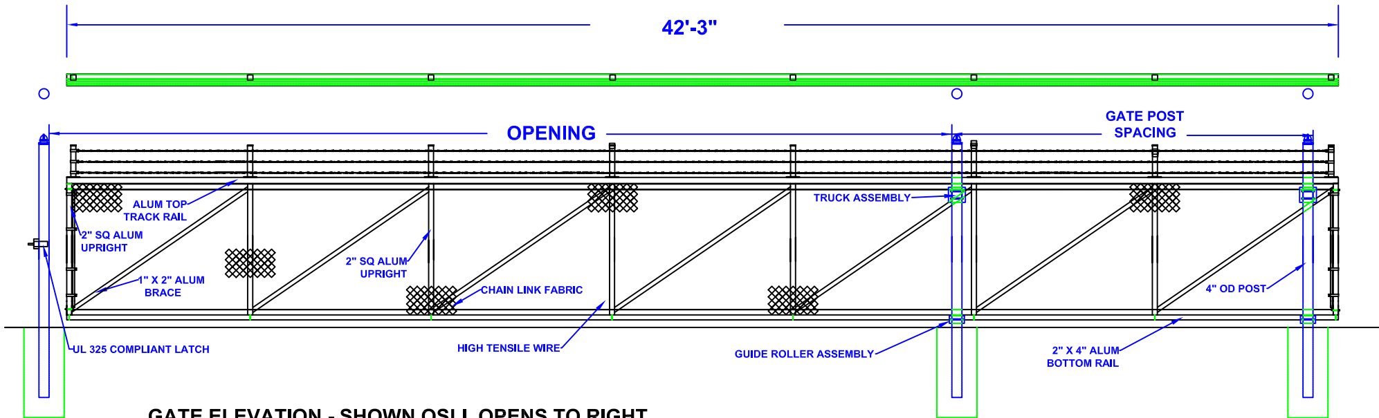
GATE ELEVATION - SHOWN OSLI, OPENS TO RIGHT UNIVERSAL DESIGN (CAN BE INSTALLED TO OPEN LEFT OR RIGHT)
